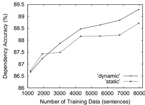
図 4 学習データと解析精度 Fig. 4 Relationship between accuracy and size of training data.
